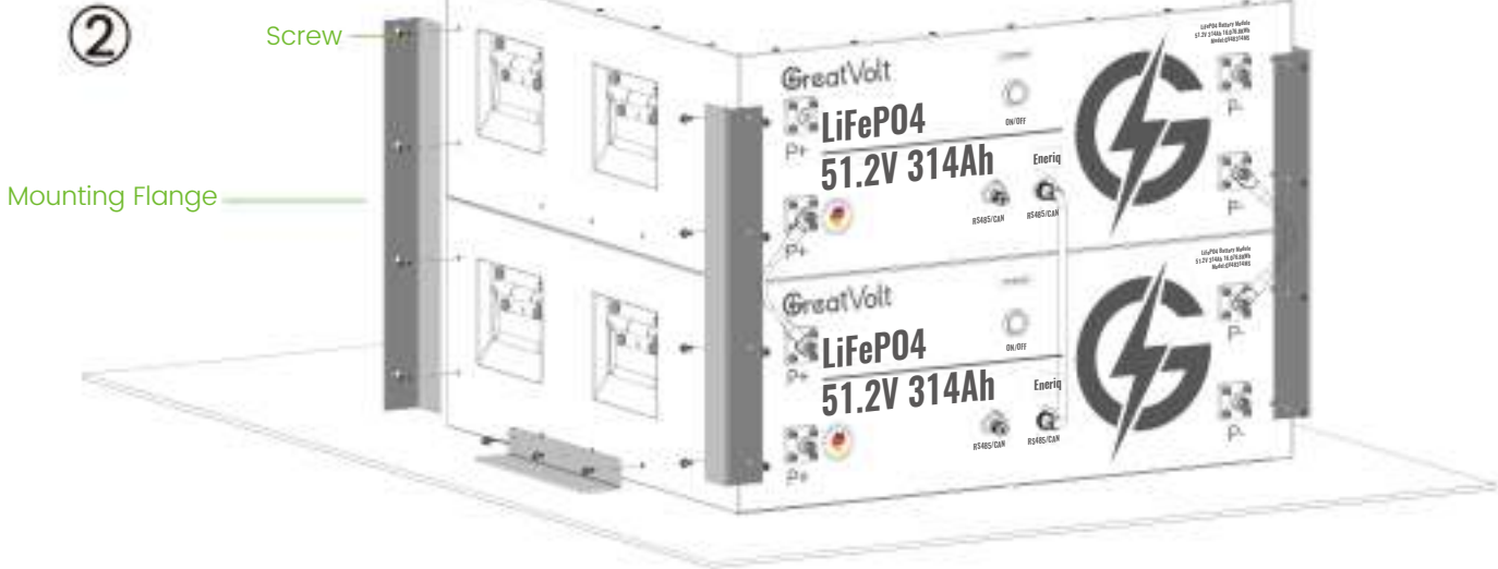
Multiple Battery Installation
