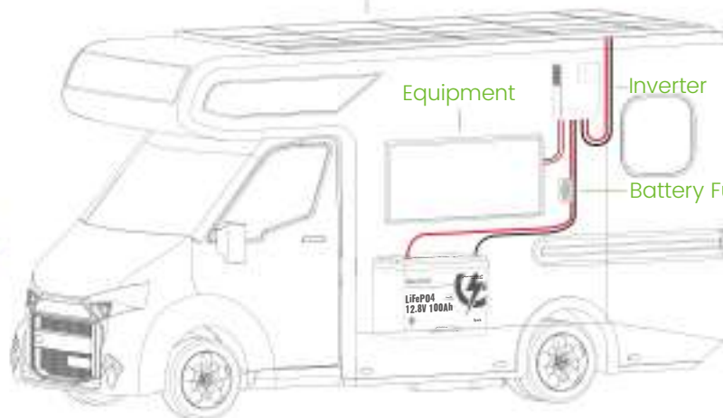
Solar panel
