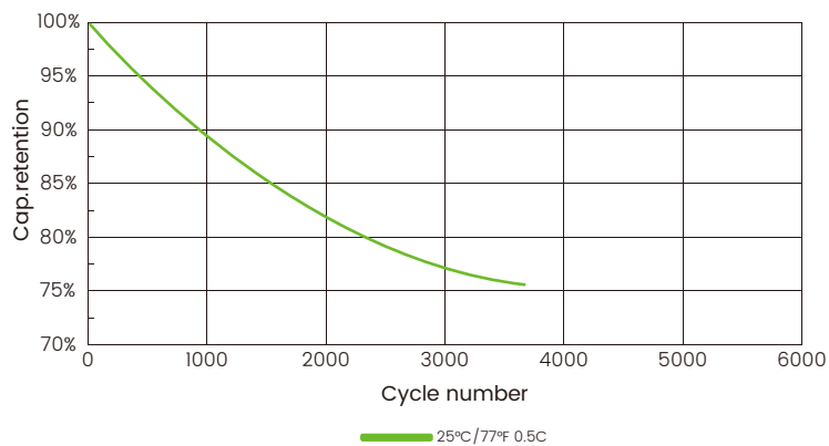
0.5C Cycle curve
